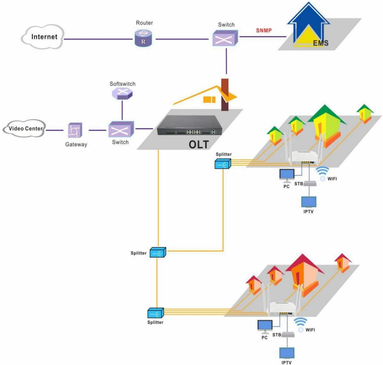
Figure: NTPL-XPON2GEACV Application Diagram
